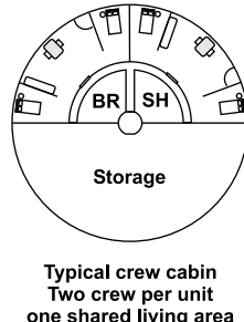
View B-B
